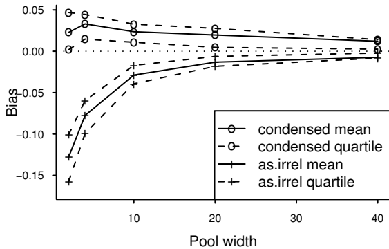
Figure 1: Empirical RBP ( p = 0.8 ) bias for unpooled system for different numbers of pooled systems. Pooling is to depth 10. The TREC 2004 Robust Track data set is used. Graphed is the mean and quartiles of the difference in mean system RBP score between the true score for the unpooled system and the score using either condensed lists or assumed irrelevance. Each data point represents 100 system set subsamplings.
