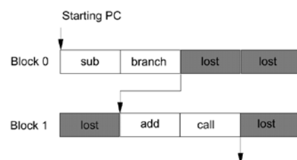
Fig. 1. Simple instructions fetch [5].
