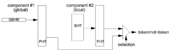
Fig. 8. Hybrid branch prediction.
