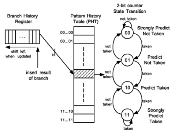
Fig. 7. 2-level adaptive branch prediction.
