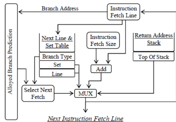
Fig. 11. NLS fetch prediction.
