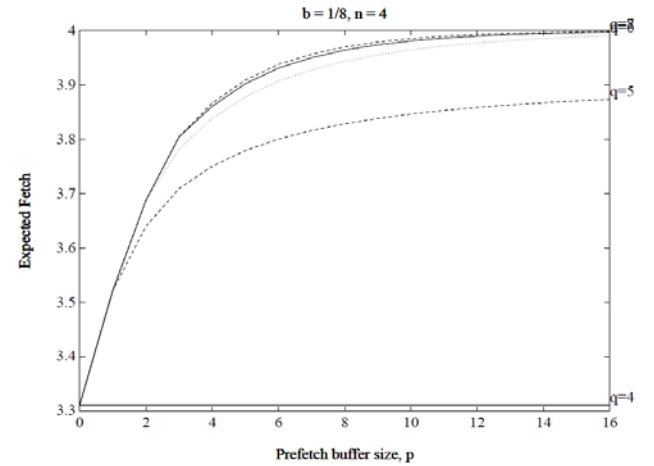
Fig. 5. Self-Aligned expected instruction fetch with prefetching ( n=4 ).
