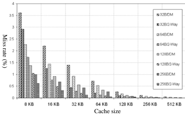
Fig. 6. Average miss rate for instruction cache with different configurations.
